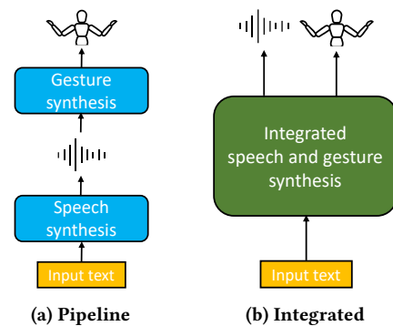
Figure 1: Two paradigms for speech and gesture synthesis.
