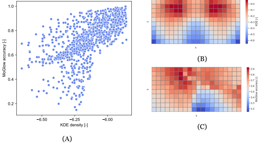
Figure 3.4: Correlation between MoGlow pointing accuracy and training data density (KDE), from Paper B. (A) Scatter plot showing strong positive correlation (Spearman r = 0.718 , p < 0.001 ). (B) KDE density and (C) MoGlow accuracy projected onto the x - z plane by averaging over y , showing that high-density training regions correspond to high-accuracy regions.
