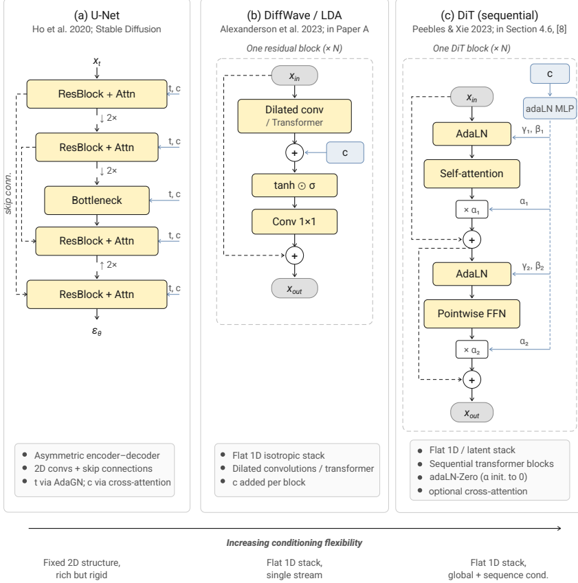
Figure 4.1: Denoising network architectures. (a) The U-Net uses an asymmetric encoder-decoder with 2D convolutions and skip connections; conditioning enters via adaptive group normalisation (AdaGN) ( t ) and cross-attention ( c ). (b) DiffWave / LDA replaces the encoder-decoder with a flat stack of residual blocks using dilated convolutions or transformers; a single temporally aligned conditioning stream is added at each block (Paper A). (c) The Diffusion Transformer (DiT) processes the sequence through sequential transformer blocks with adaLN-Zero conditioning and optional cross-attention, supporting both global and sequence-level signals (Section 4.6). The progression from left to right reflects increasing conditioning flexibility.
