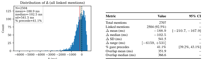
(a) Distribution of gaze-speech lag \Delta (fixation offset minus mention onset). Negative values ( \Delta < 0 ) indicate that the fixation ended before mention onset; positive values indicate temporal overlap.
