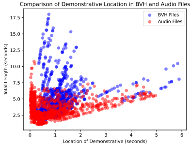
Figure 3: Demonstrative location against total length (in seconds) for motion (BVH) and audio files.
