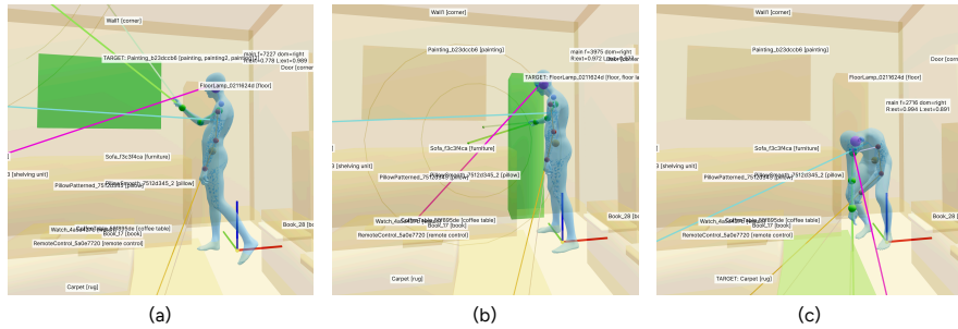
Figure 6.6: Gesture reference visualizer in the Viser-based tool. Each panel shows the SMPL-X mesh with object bounding boxes (green). (a) Pointing toward a painting (Tier 1: clear alignment). (b) Pointing toward a floor lamp with the target bounding box highlighted. (c) Bending gesture toward the carpet, illustrating a less canonical pointing pose.
