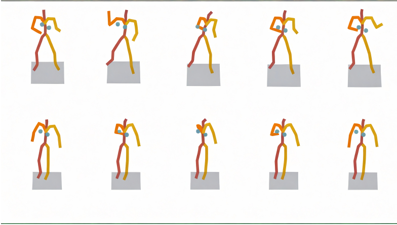
Figure 4.3: Qualitative effect of fine-tuning on pointing data. Top: the base OmniControl model reaches the target wrist position with a punching motion. Bottom: after fine-tuning on the pointing gesture corpus, the same spatial target elicits a natural pointing gesture. Both sequences are generated from the same conditioning input; only the training data differs.
