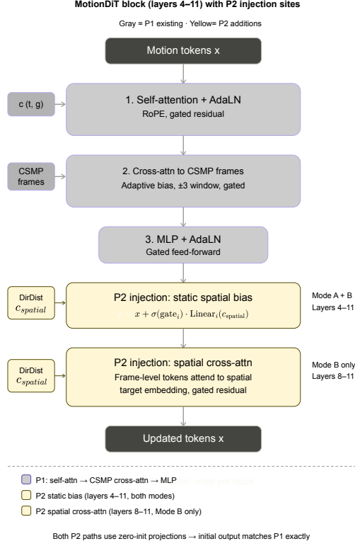
Figure 4.4: Single MotionDiT transformer block (layers 4–11) showing P1 co-speech components (gray) and P2 spatial injection sites (yellow). The spatial pathway adds a gated residual bias on layers 4–11 (Mode A and B) and single-token cross-attention on layers 8–11 (Mode B only). Both paths use zero-initialized projections, so the initial P2 output matches P1 exactly.
