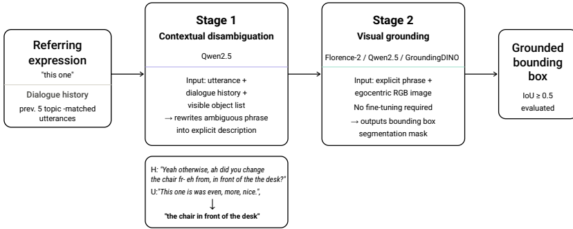
(a) Two-stage rewrite-based grounding pipeline.
