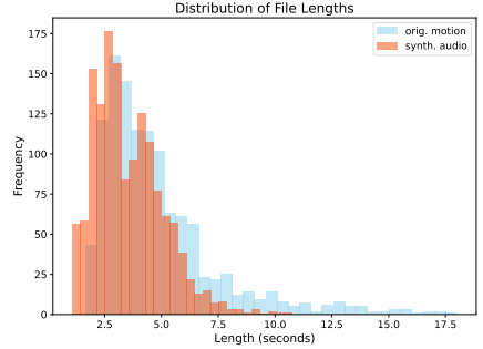
Figure 1: Distribution of length of pointing motion clips and synthesized audio clips.
