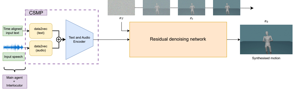
Figure 2: Architecture of the motion synthesis module
