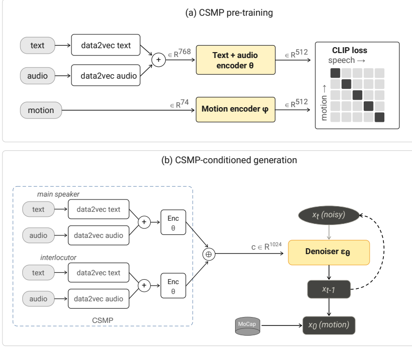
Figure 4.2: Architecture of the Contrastive Speech and Motion Pretraining (CSMP) module and its integration into the diffusion-based generation pipeline (Paper A). (a) During pre-training, data2vec representations of text and audio are summed and encoded by a transformer-based speech encoder \theta , while a motion encoder \varphi processes raw pose vectors. The two encoders are trained with a symmetric contrastive (CLIP) loss. (b) At generation time, the pre-trained encoder \theta produces embeddings for both the main speaker and the interlocutor, which are concatenated into a conditioning signal c \in \mathbb{R}^{1024} that guides the classifier-free diffusion denoiser.
