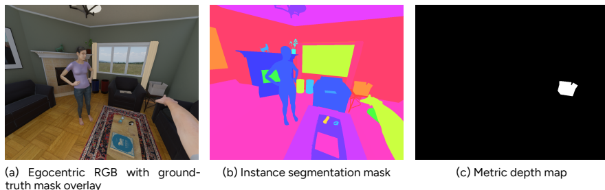
Figure 5.1: A grounded data sample from MM-Conv. For the referring expression box, the dataset provides (a) the egocentric RGB view with the ground-truth referent highlighted, (b) the per-pixel instance segmentation mask, and (c) the corresponding depth map. Word-level timestamps link the expression to this exact simulator frame. Rendered in Blender.
