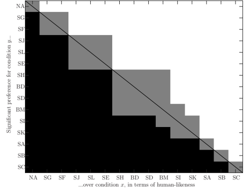
Figure 4: Significance of pairwise differences between conditions. White means the condition listed on the y -axis achieved an MAS significantly above the condition on the x -axis, black means the opposite ( y scored below x ), and grey means no statistically significant difference at level \alpha = 0.05 after correction for the false discovery rate. Conditions use the same order as the corresponding subfigure in Figure 3
