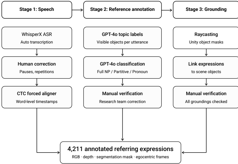
Figure 6.5: Annotation pipeline for the MM-Conv dataset. Each stage combines automated processing with manual verification.
