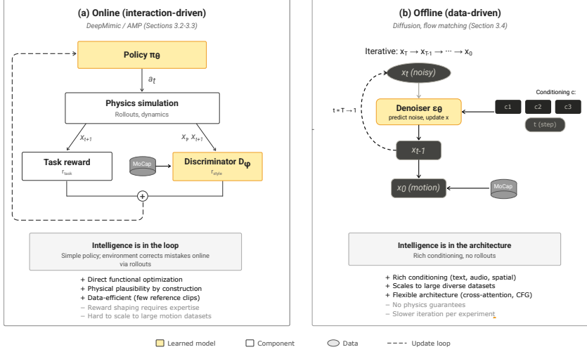
Figure 3.3: Structural contrast between the two generative paradigms used in this thesis. Online methods (a) employ a simple policy within a physics simulation loop, where the environment provides information; offline methods (b) employ a deep generative model trained on fixed data, where conditioning enters through architectural pathways (cross-attention, adaLN).
