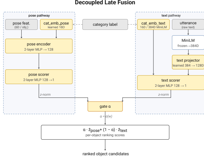
Figure 5.3: PoseRefer architecture. Pose and text pathways operate independently with no shared parameters. Each pathway has its own per-object category embedding table (learned 16-D for pose, frozen MiniLM 384-D for text). Per-pathway scores are z-normalized and combined by a learned scalar gate \alpha . The decoupling makes pathway contributions directly ablatable: disabling category on one pathway leaves the other unchanged.
