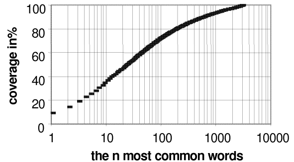
Figure 1. Word coverage as a function of frequency.
